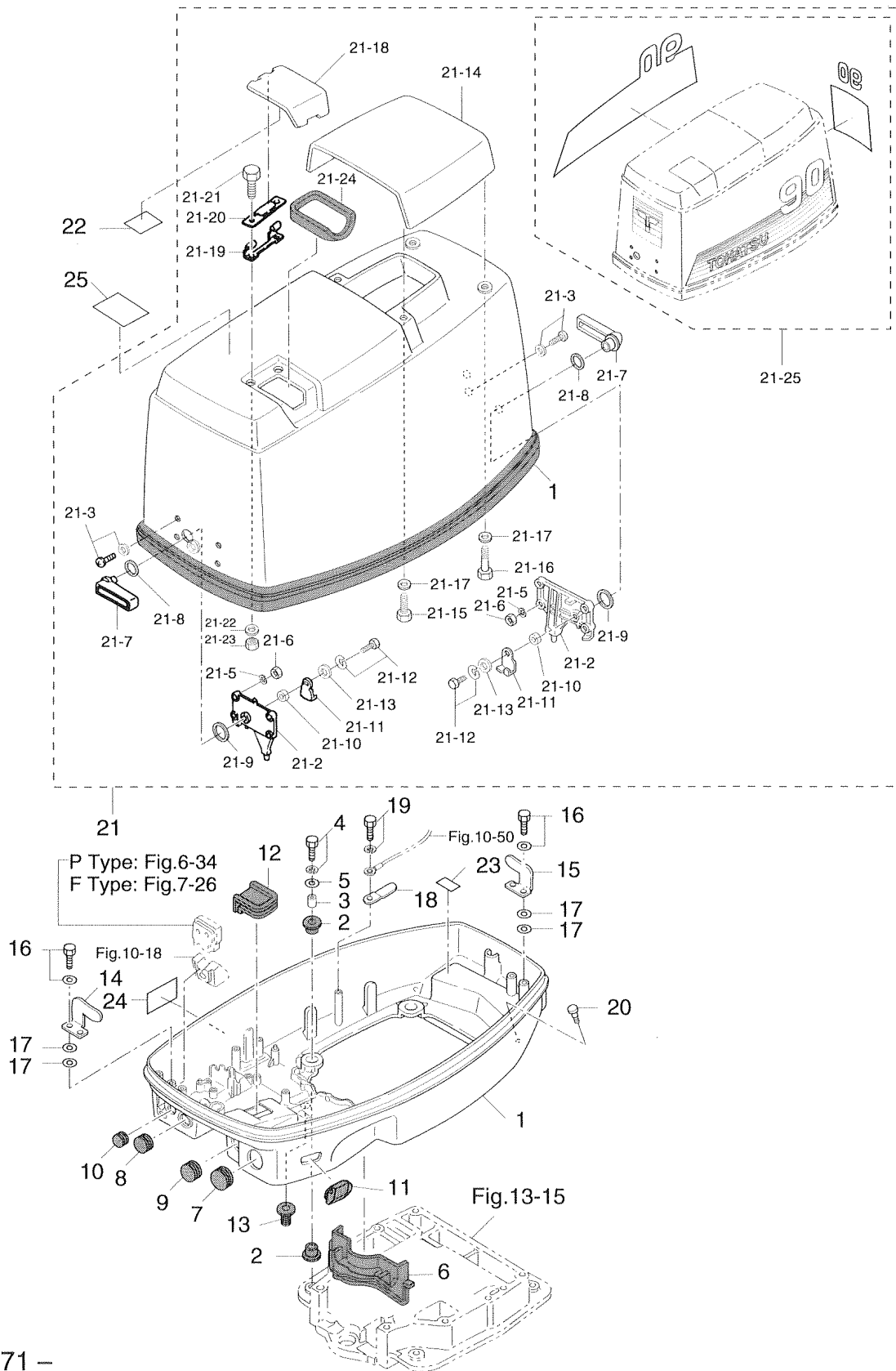
Fig. 21 MOTOR COVER
