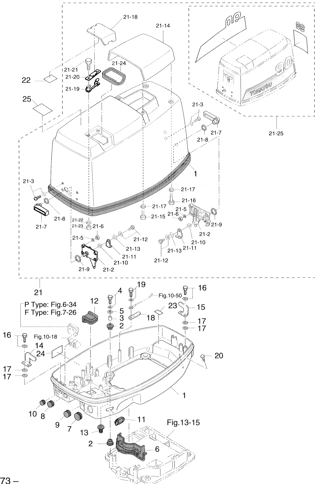
Fig. 21 MOTOR COVER (cont.)
