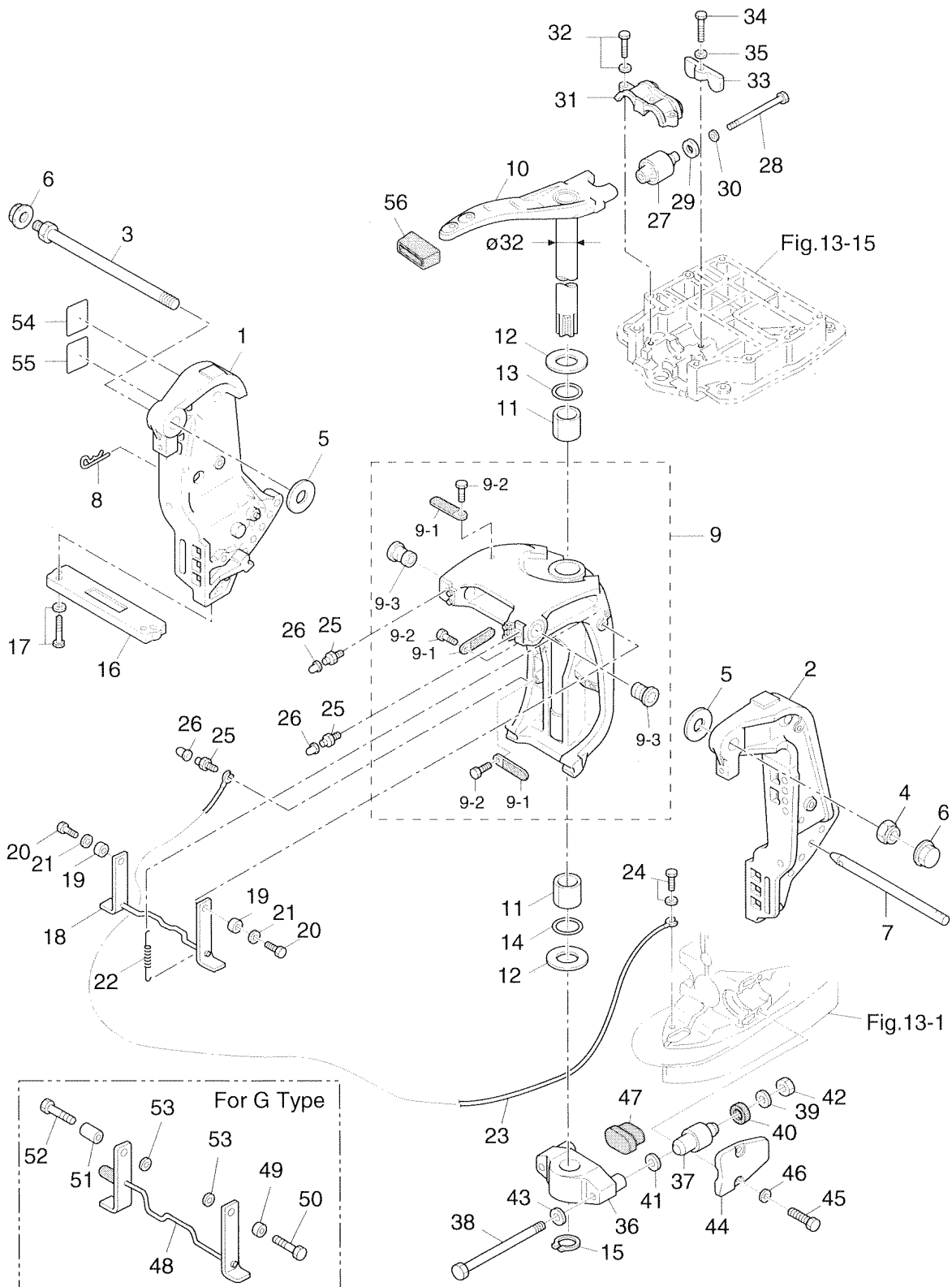
Fig. 17 BRACKET
