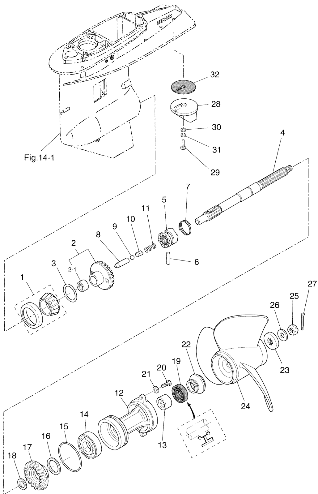
Fig. 15 GEAR CASE (PROPELLER SHAFT) (cont.)
